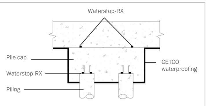
Figure 5.2 - Waterstop-RX encircling pile caps metal reinforcement
