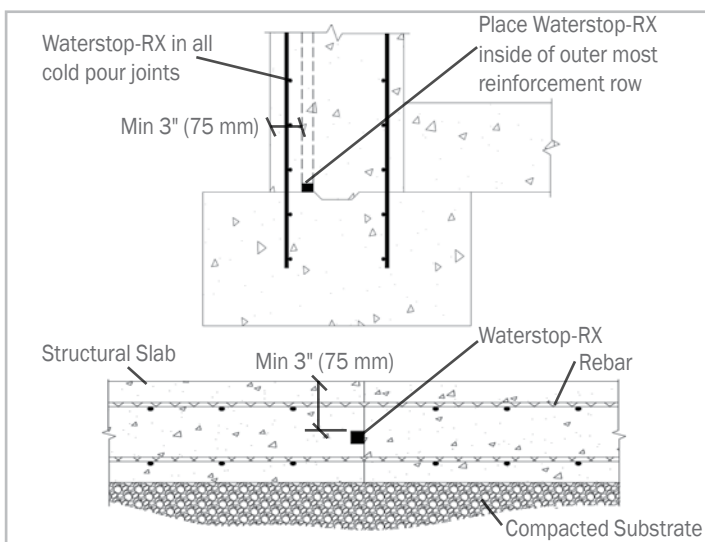
Figure 3.1 - Placement of Waterstop-RX 101 & 101T at typical construction joints with required 3" (75 mm) concrete coverage.
