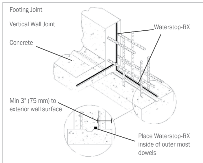
Figure 2.1 - Typical placement of Waterstop-RX at concrete construction joint
