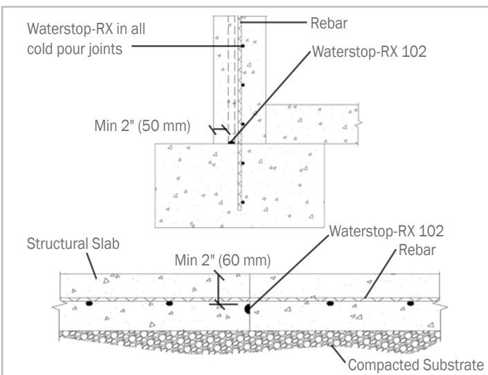
Figure 3.2 - Placement of Waterstop-RX 102 at typical construction joints with required 2" (50 mm) concrete coverage.
